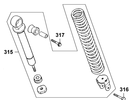
F17 Rear Cushion
